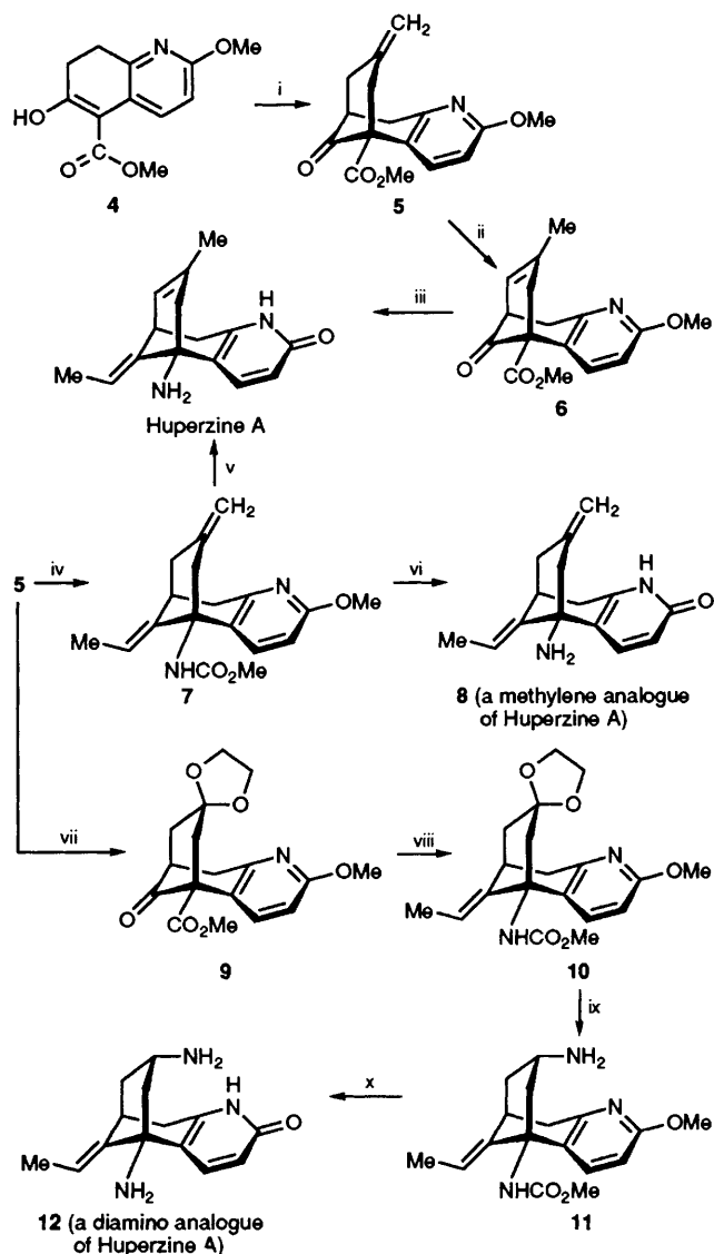
Scheme 2 Reagents and conditions: i, 2-methylenepropane-1,3-diol diacetate, Pd(OAc) 2 , PPh 3 , 1,1,3,3-tetramethylguanidine, dioxane (92%); ii, TfOH, dioxane, 93 °C, resealable tube (90%); iii, same steps as reported in ref. 4; iv, a, Ph 3 P=CH=Me, tetrahydrofuran (THF) (83%); b, PhSH, azoisobutyronitrile, PhMe, 85 °C (92%); c, 20% NaOH, MeOH, THF, reflux (83%); d, (PhO) 2 PON 3 , Et 3 N, PhMe, reflux; MeOH, reflux (82%); v, a, TMSI, CHCl 3 , reflux; MeOH, reflux; b, TfOH, dioxane, 93 °C, resealable tube (84% for the two steps); vi, Pr n SLi, HMPA, 90 °C (87%); vii, a, OsO 4 , 80% HOAc; NaIO 4 , (89% overall); b, ethylene glycol, toluene- p -sulfonic acid ( p -TSA), benzene, reflux (94%); viii, conditions of iv (88%, 94%, 81%, and 80% for the respective steps); ix, a 5% HCl, Pr n OH, 70 °C (93%); b, NH 3 , MeOH, NH 4 Cl, 70 °C, resealable tube; NaBH 4 , 0 °C (84%); x, TMSI, CHCl 3 , reflux; MeOH, reflux (82%)
