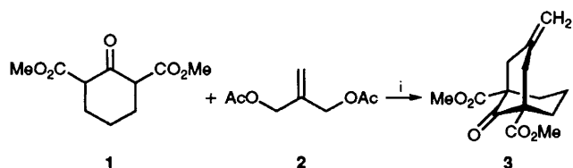
Scheme 1 Reagents: i, Pd(OAc) 2 , ethylenebis(diphenylphosphine), N,O -bis(trimethylsilyl)acetamide
